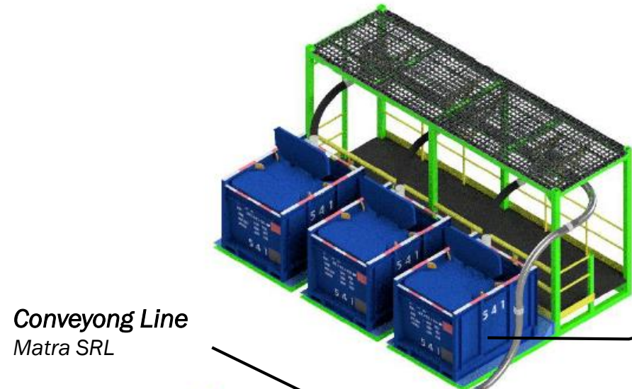
Cutting box Client/Matra SRL
