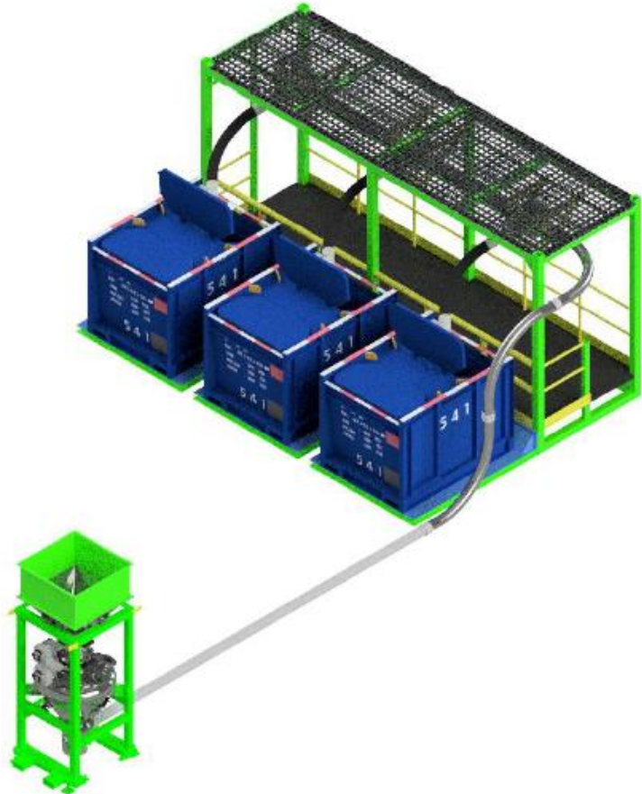
General Arrangement - Waste Management Offshore Plant
