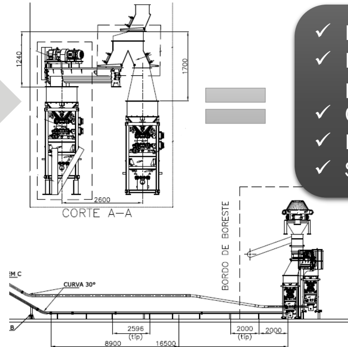
Layout 2 - Double Pneumatic Transporter for Cutting and Solids Handling on Drillship
