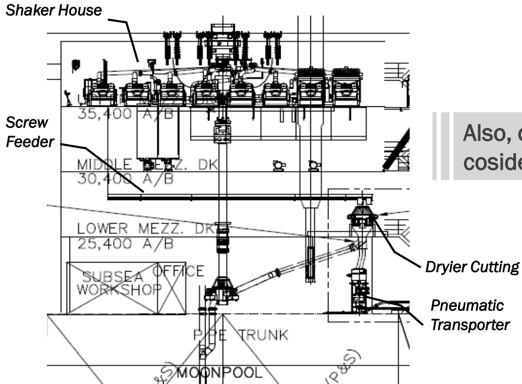
Layout 1 - Cutting and Solids Handling on Drillship
